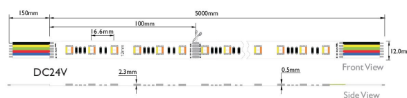
Dimensions(Unit: mm)
