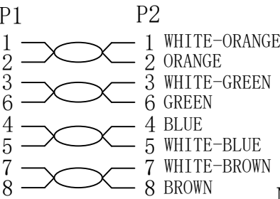
WIRING DIAGRAM
